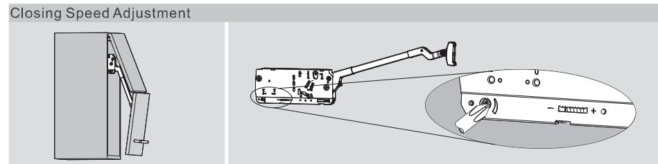
"+" increasing soft-closing time (turn adjustment screw counter-clockwise) "-" reducing soft-closing time (turn adjustment screw clockwise)
