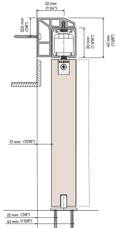
Perfil soporte pared 17 mm Wall Support Profile 17mm | Profile Support Mural 17 mm
